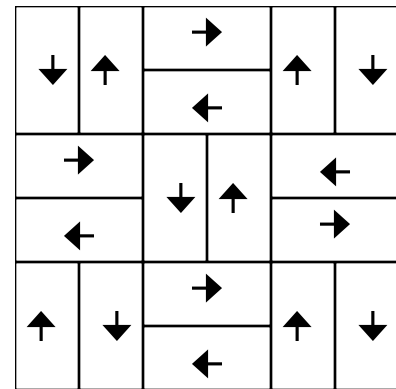
Shuffled/Random
