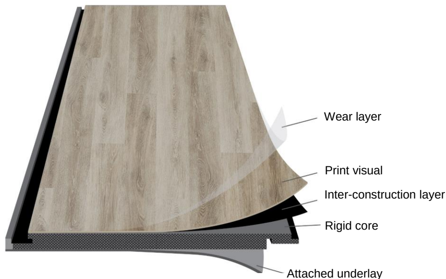
Figure 1: Diagram of rigid core flooring cross section
